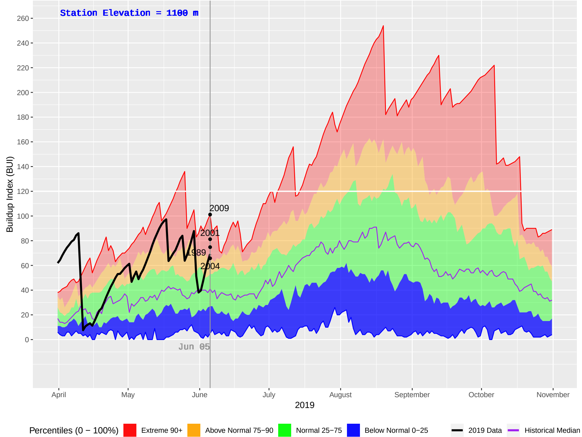
PALLISER (411) : Historical (1973–2018), Current (2019) Daily Buildup Index (BUI)
