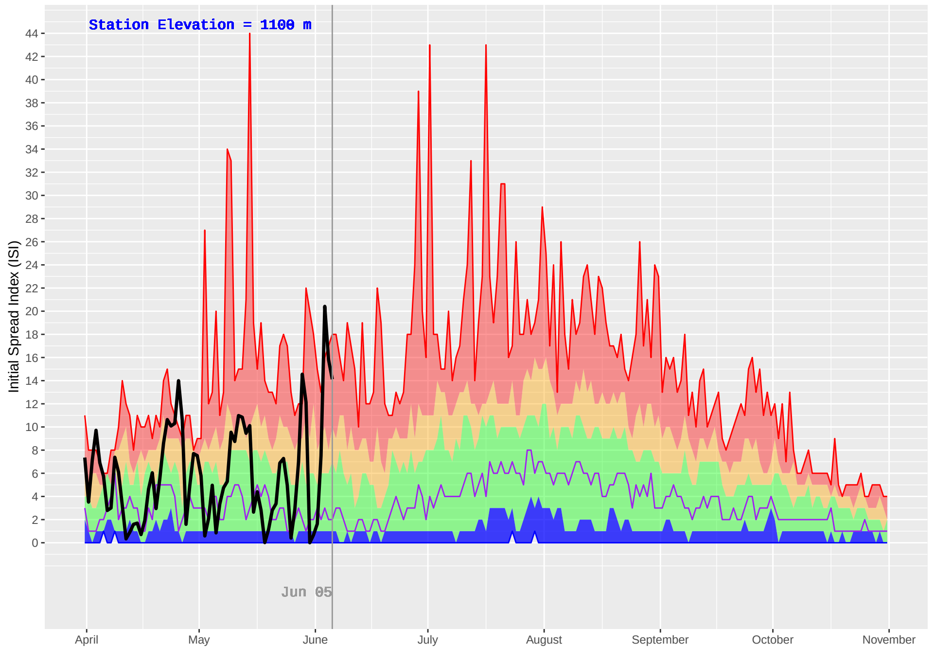
PALLISER (411) : Historical (1973–2018) and Current (2019) Daily Initial Spread Index (ISI)
