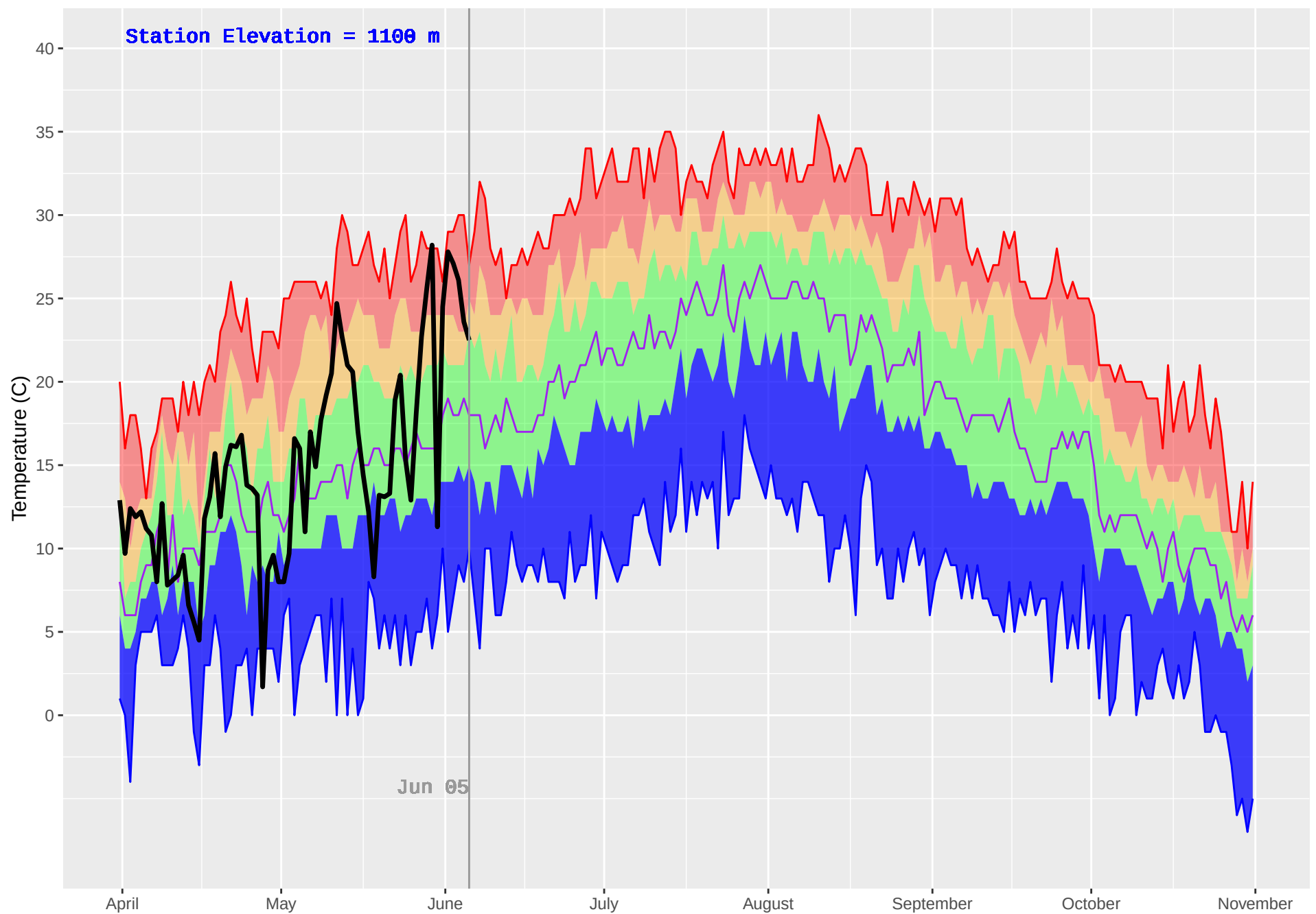
PALLISER (411) : Historical (1973–2018) and Current (2019) Daily Temperature
