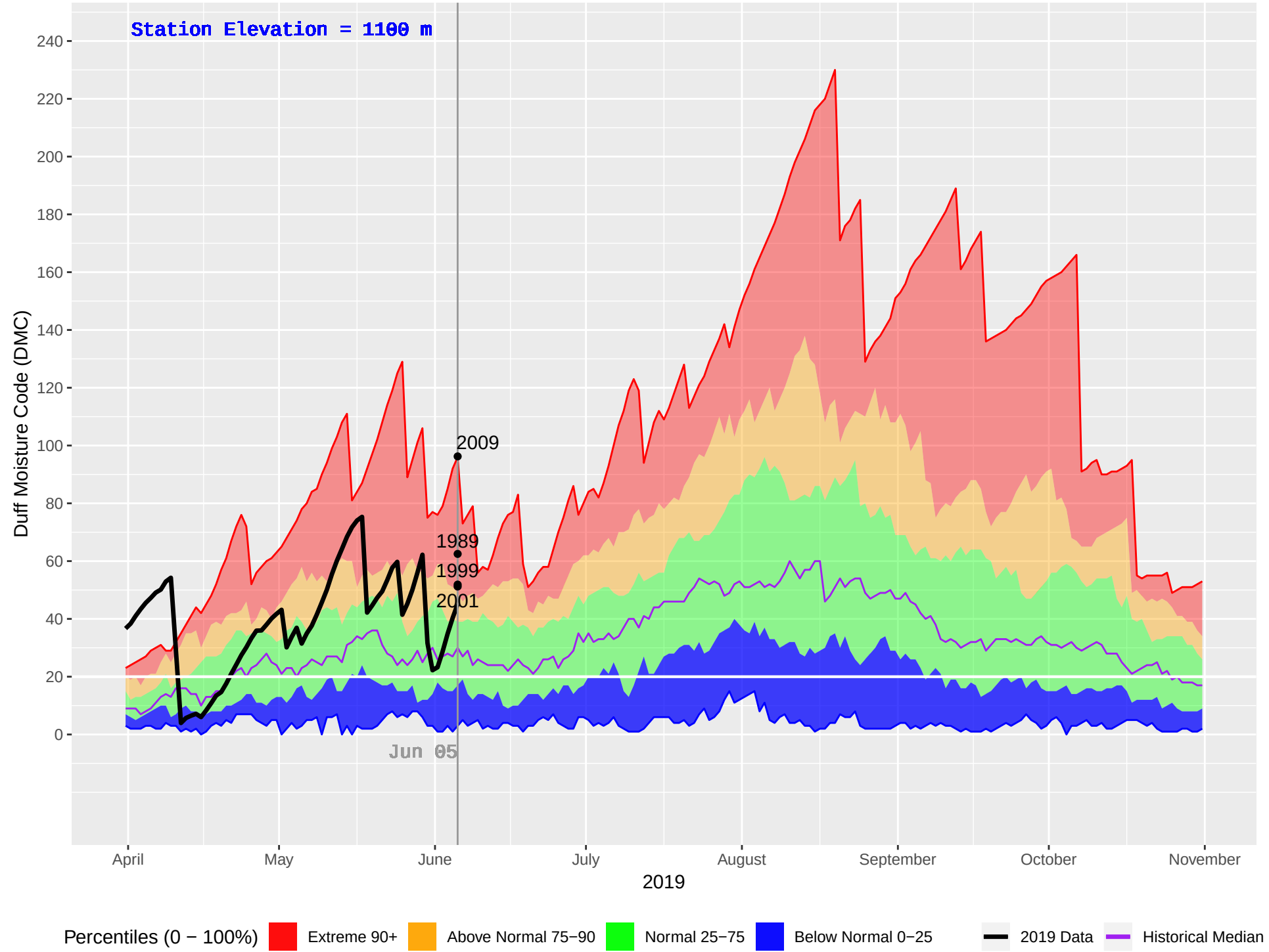
PALLISER (411) : Historical (1973–2018), Current (2019) Daily Duff Moisture Code (DMC)
