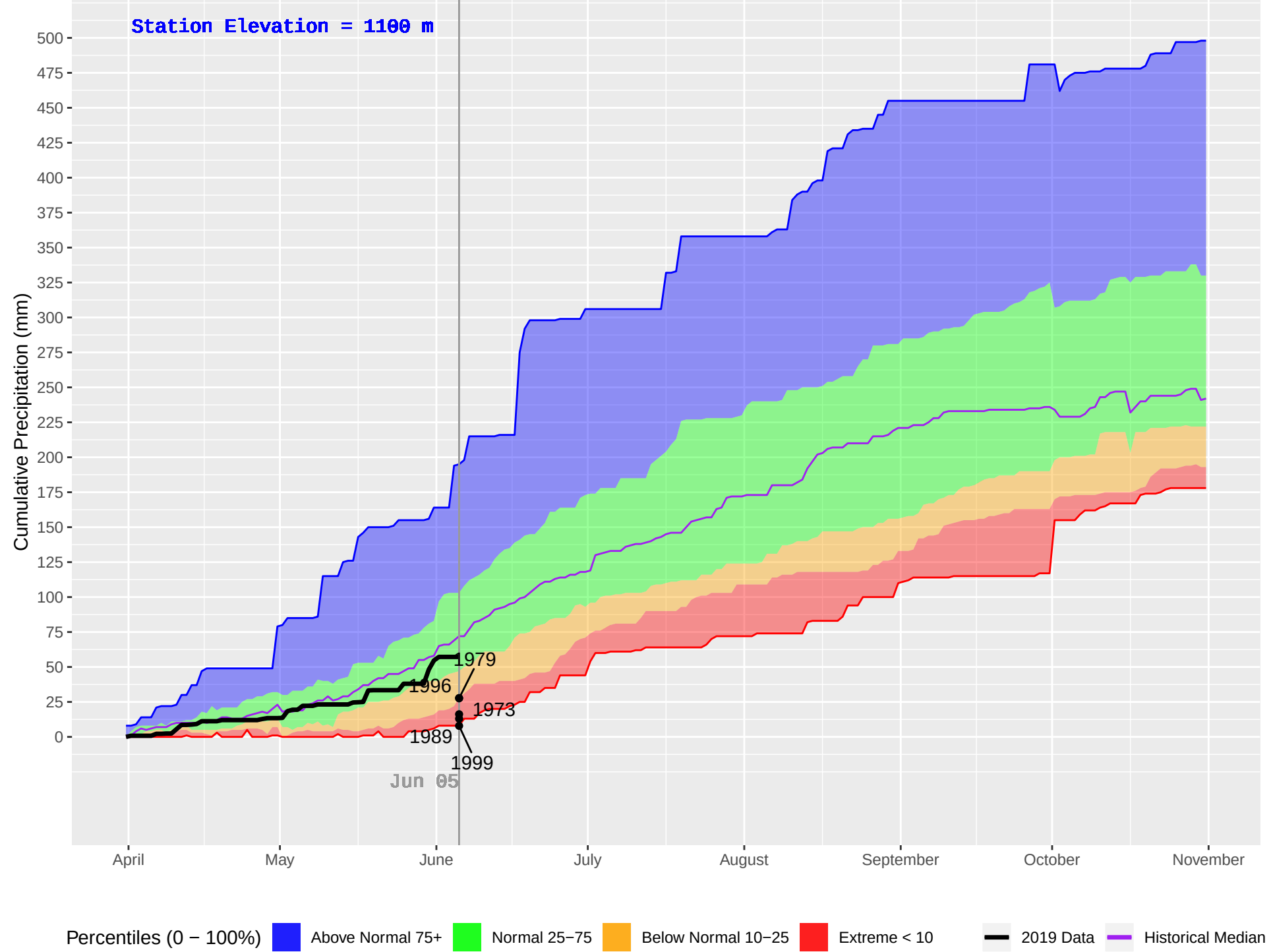
PALLISER (411) : Historical (1973–2018), Current (2019) Daily Cumulative Precipitation
