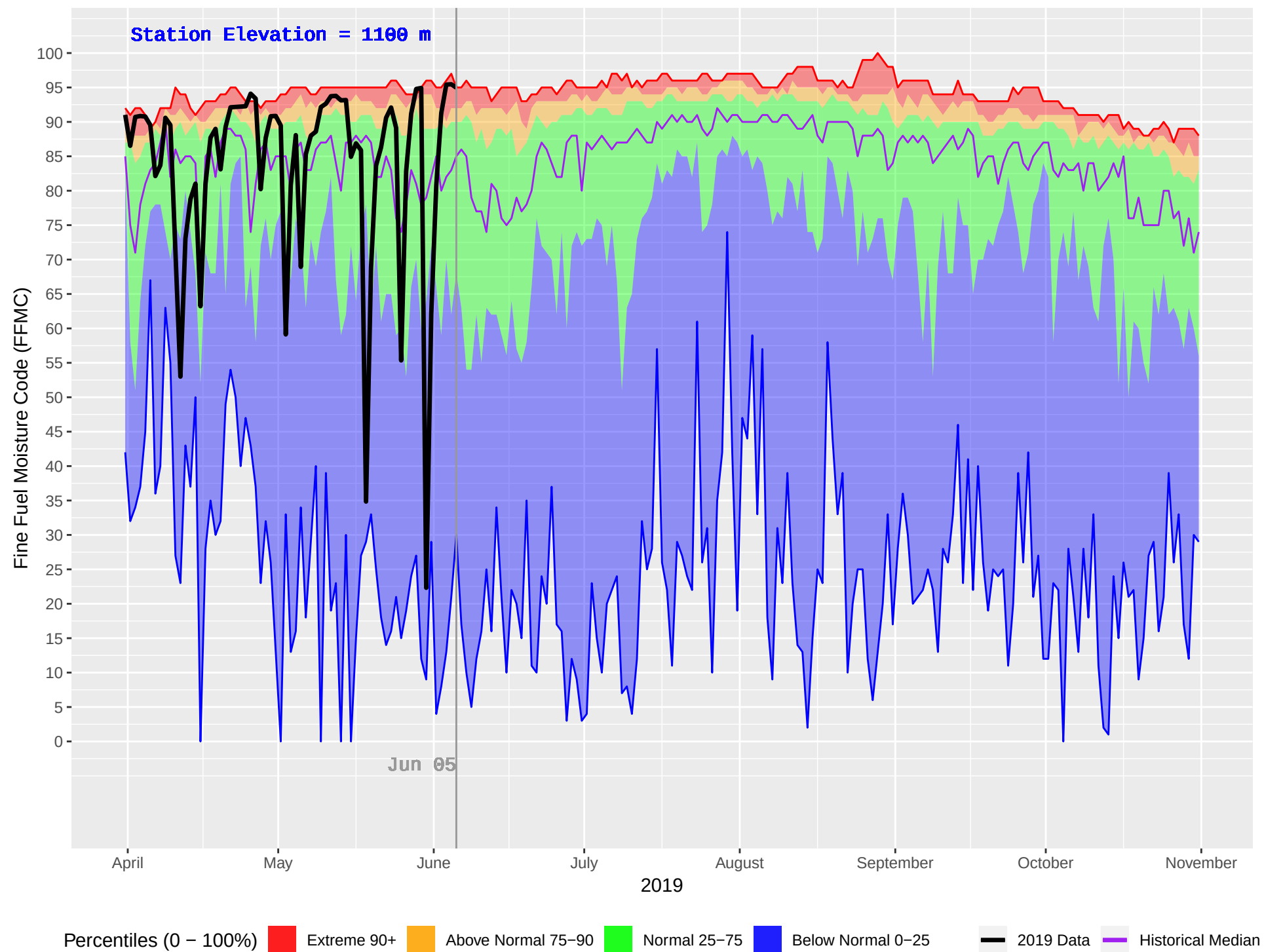
PALLISER (411) : Historical (1973–2018) and Current (2019) Daily Fine Fuel Moisture Code (FFMC)
