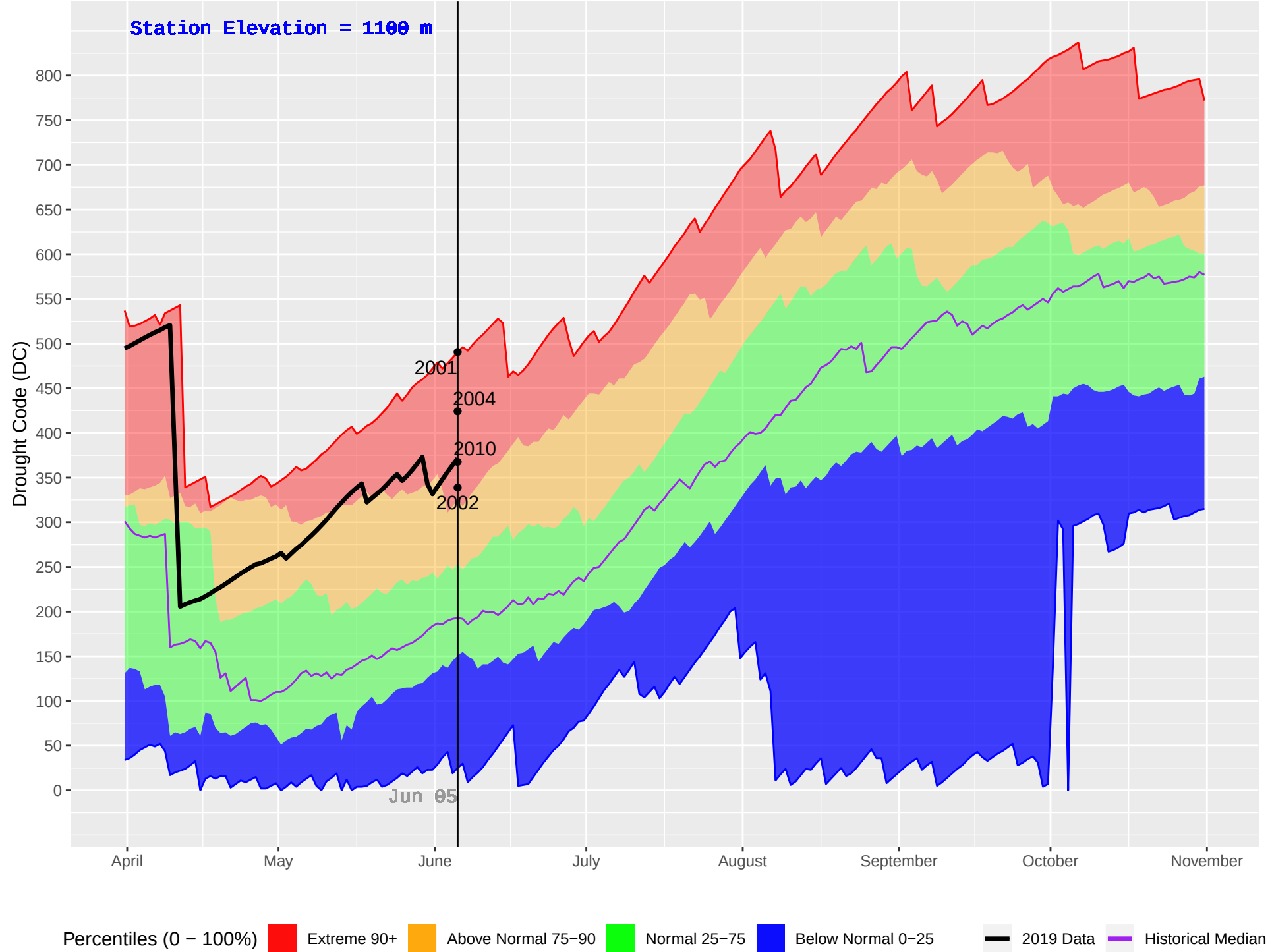
PALLISER (411) : Historical (1973–2018) and Current (2019) Daily Drought Code (DC)
