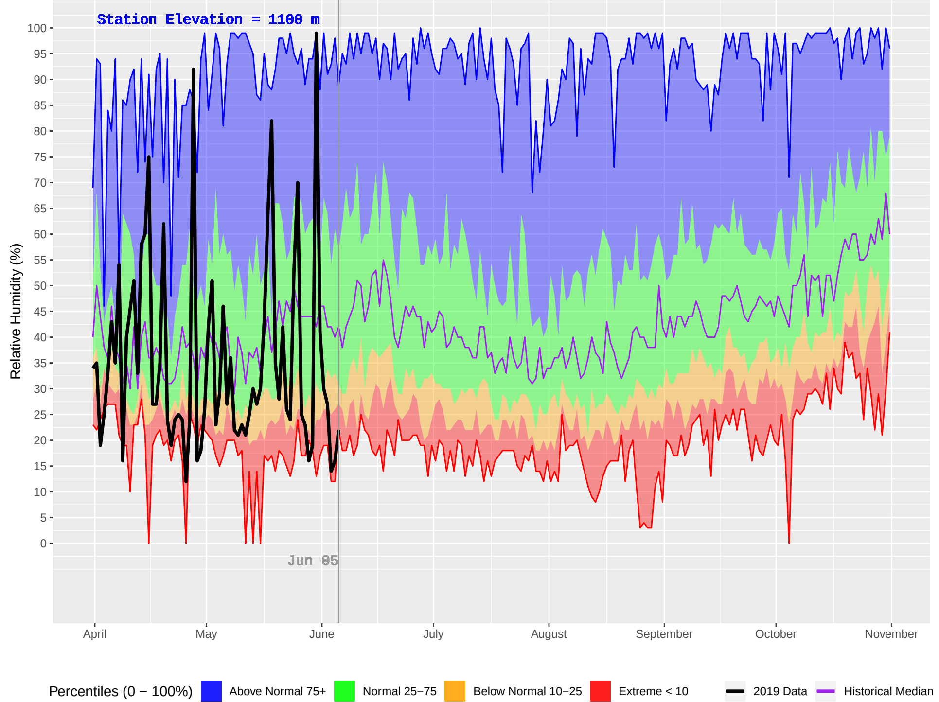
PALLISER (411) : Historical (1973–2018) and Current (2019) Daily Relative Humidity
